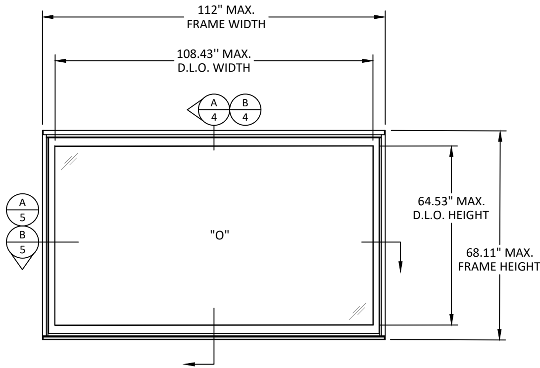
ELEVATION FIXED WINDOW
